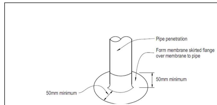
Figure 28: Pipe penetrations
