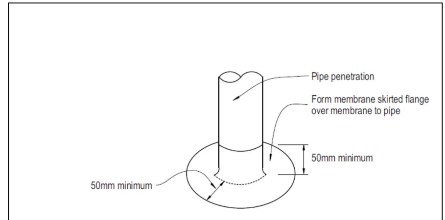
Figure 28: Pipe penetrations
